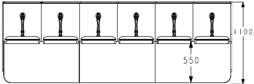
TOP VIEW
