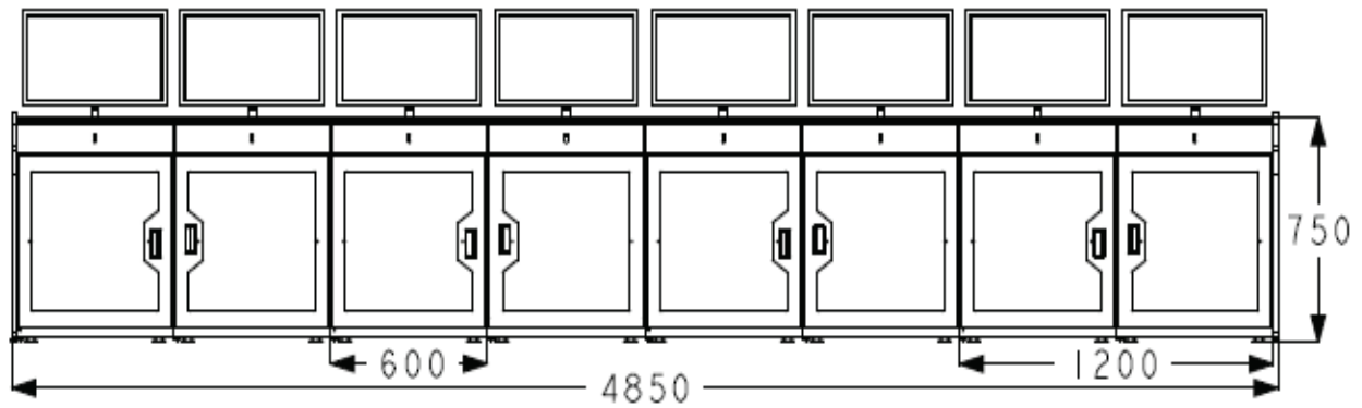
FRONT VIEW
