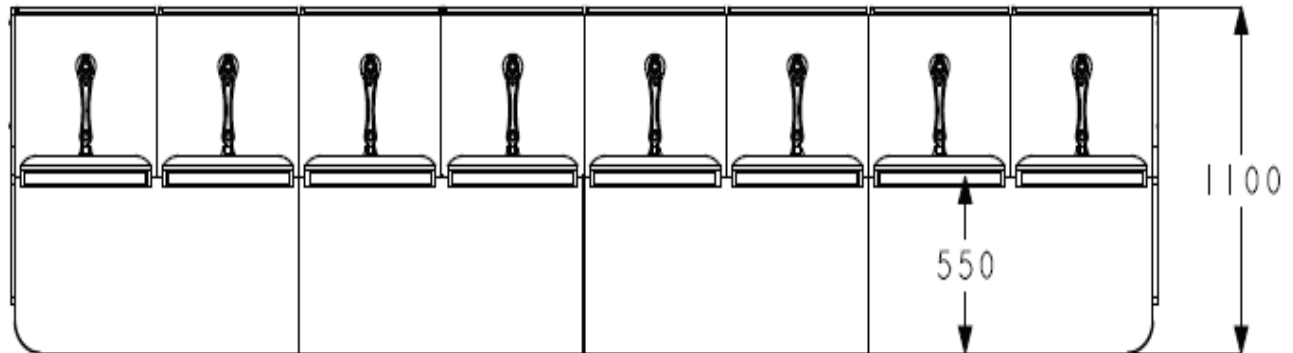
TOP VIEW
