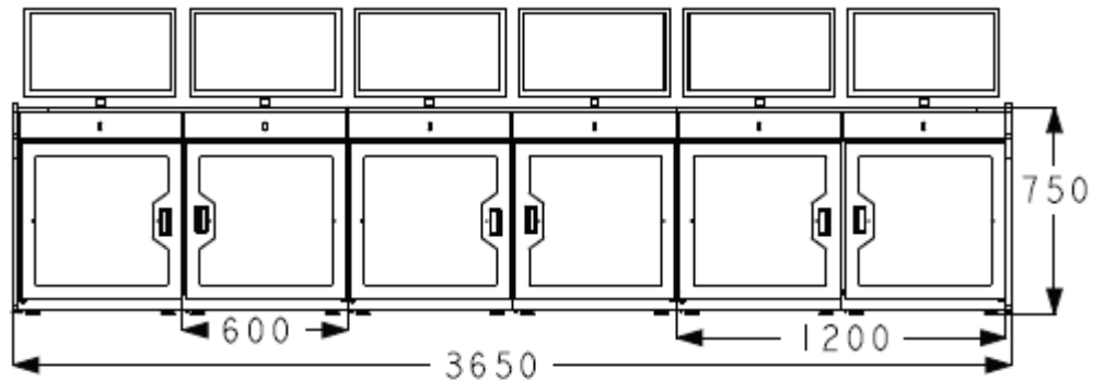
FRONT VIEW
